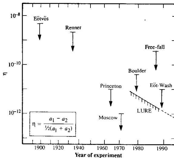
Fig. 2. Selected tests of the Weak Equivalence Principle, showing the bounds on \eta , which measures the fractional difference in acceleration a of different materials or bodies. The free-fall and Eöt-Wash experiments were originally performed to search for the fifth force. Hatched and dashed lines show current and projected bounds, respectively, on \eta for gravitating bodies (test of the Strong Equivalence Principle) from lunar laser ranging (LURE). For discussion and references, see (8).
