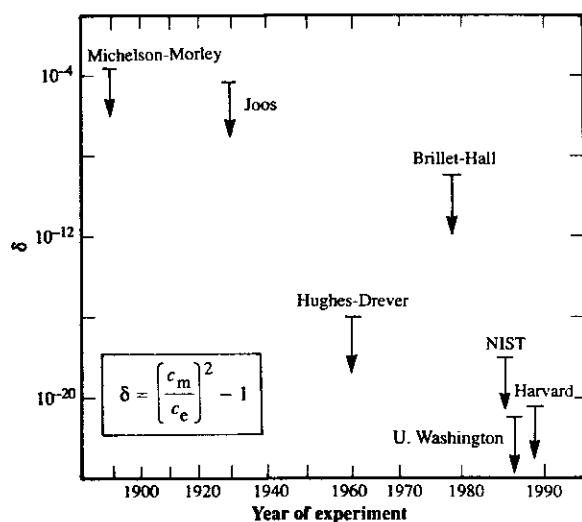
Fig. 1. Selected tests of SR showing the bounds on the parameter \delta , which measures the degree of violation of Lorentz invariance in electromagnetism. The Michelson-Morley, Joos, and Brillat-Hall experiments test the isotropy of the round-trip speed of light, the Brillat-Hall experiment using laser technology. The remaining four experiments test the isotropy of nuclear energy levels. Limits assume an Earth speed of 300 \text{ km s}^{-1} relative to the mean rest frame of the universe; NIST, National Institute of Standards and Technology. For discussion and references, see (11).
