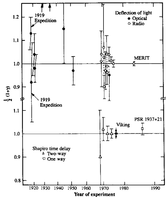
Fig. 3. Measurements of the coefficient (1 + \gamma)/2 from light deflection and Shapiro time delay measurements. The GR value is unity. Arrows at the top margin denote anomalously large values from the 1929 and 1936 expeditions. Shapiro time delay measurements using the Viking spacecraft yielded (1 + \gamma)/2 = 1.000 \pm 0.001 . For discussion and references see (32, 43, 45).
